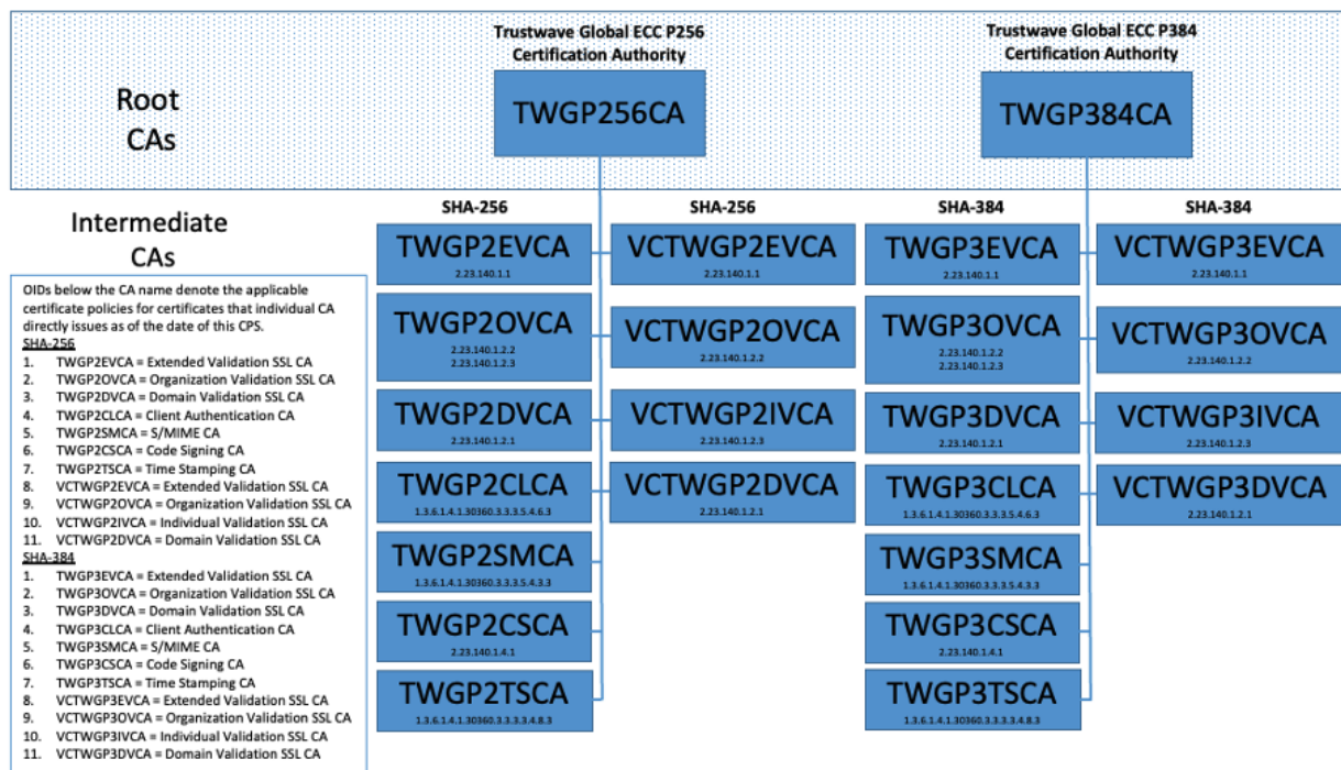
Figure 1 - The VikingCloud Public Key Infrastructure
