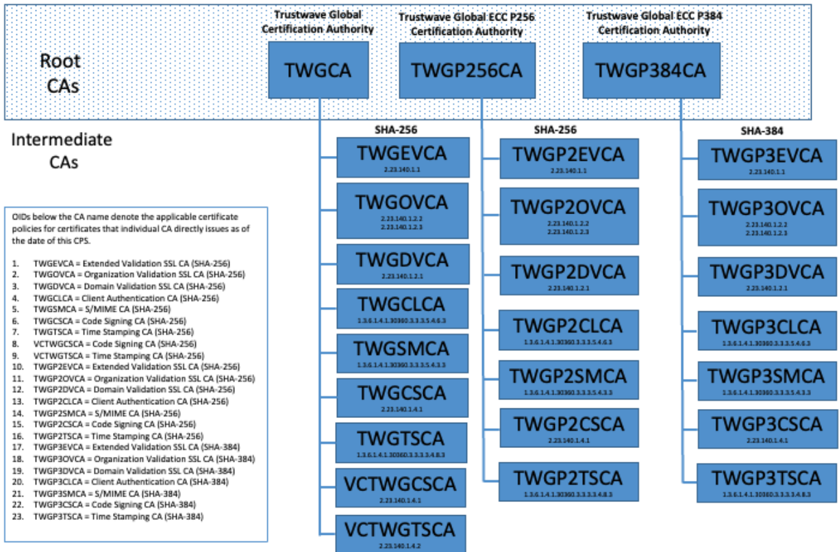
Figure 1 - The VikingCloud Public Key Infrastructure
